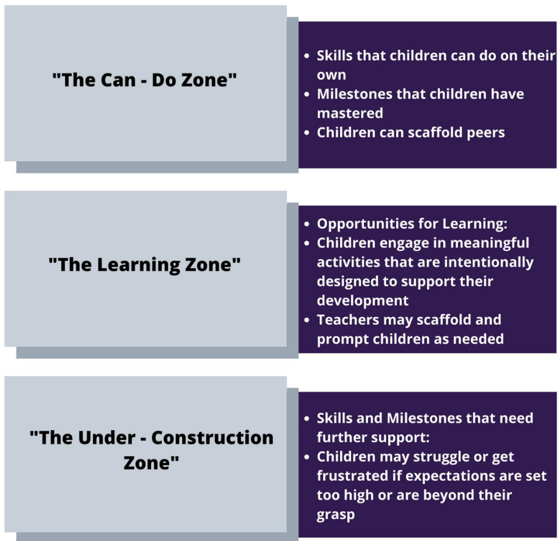
Figure 5.4 Learning Zones. 60
