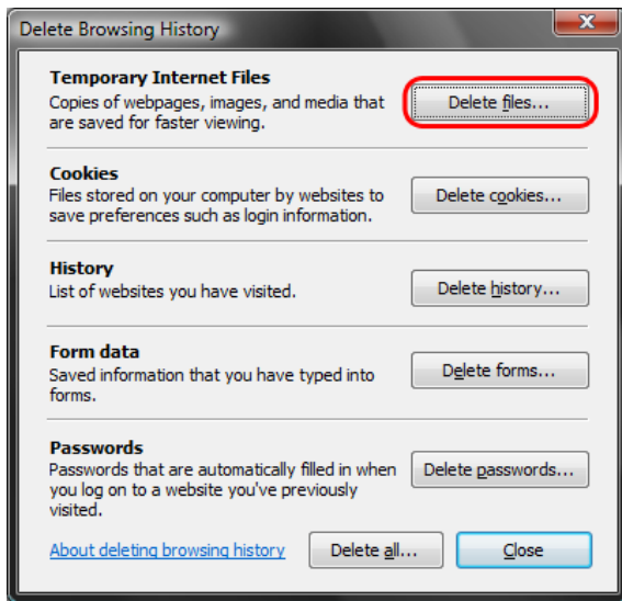
Internet Explorer 7
