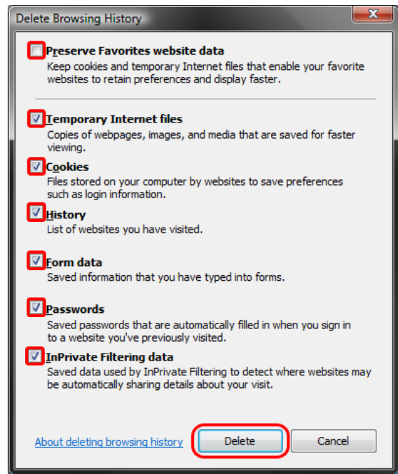
Internet Explorer 8
